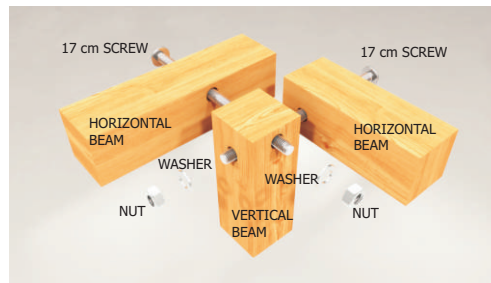
VERTICAL AND HORIZONTAL BEAM CONNECTION (FLOOR AND ROOF SITUATION)
